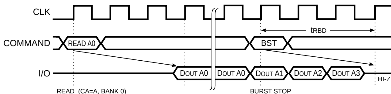
CAS latency = 3, burst length = full page
