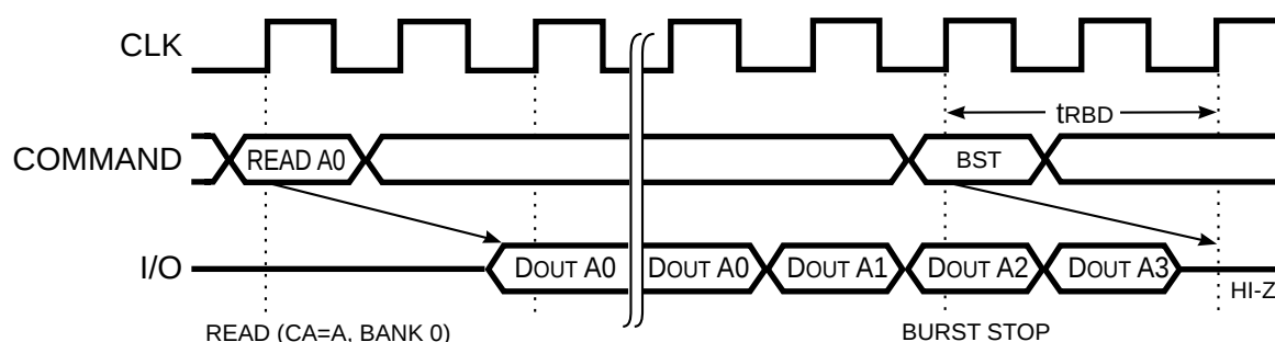
CAS latency = 2, burst length = full page
